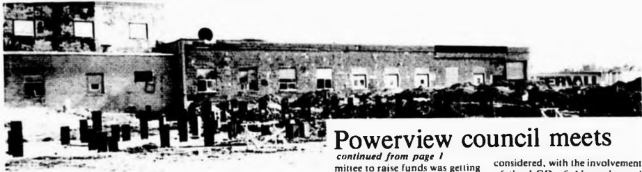
Construction of a warehouse behind the Abitibi-Price paper mill has been underway since May and expected completion date is late September. These steel piles will have backfill before an on grade concrete slab is poured. The steel warehouse will have a capacity of 4000 tons and will house offices for paper machine personnel, engineering and control as well as storage for paper.
